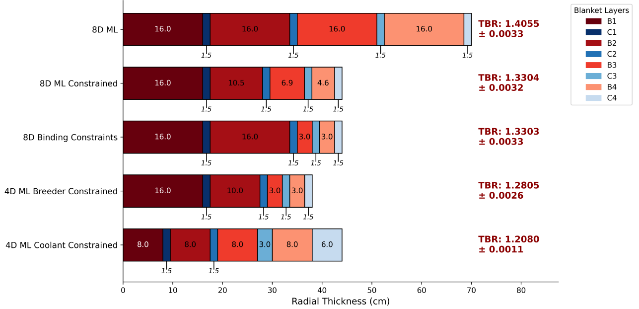
Figure 11: Radial thickness profiles and resulting global TBR for the ML optimised TBR-thickness studies detailed in Section 4.3.3. Associated TBR values are annotated alongside their standard statistical uncertainty. N = 100 was used for all except for unconstrained 8D N = 150 , where these include N_{sobol} = 50 . Hyper-parameters \epsilon = 0.5 and \beta = 1,000,000 were tuned for these studies.
