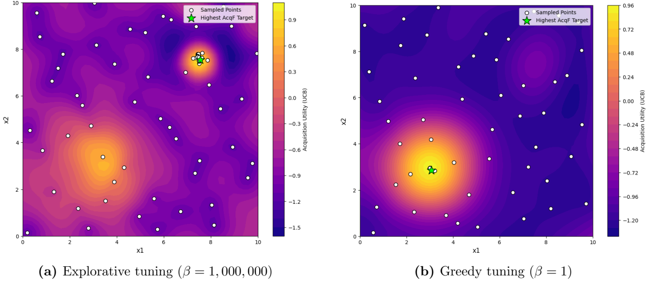
Figure 3: Comparison of the Upper Confidence Bound (UCB) acquisition function behaviour under different exploration parameters ( \beta ). (a) A high \beta value successfully prioritises exploration, identifying a secondary hidden peak. (b) A low \beta value results in overly greedy exploitation, causing the model to stagnate on a single local optimum and ignore unexplored regions.
