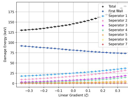
Figure B3: Total damage energy deposited into the plasma-facing FW and internal structural separators across the geometric gradient.
